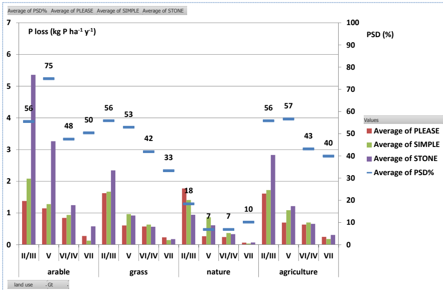
Figure 1. The measured average PSD, and estimates of the average annual P losses according to the PLEASE and SIMPLE approaches and the STONE dynamic model.
