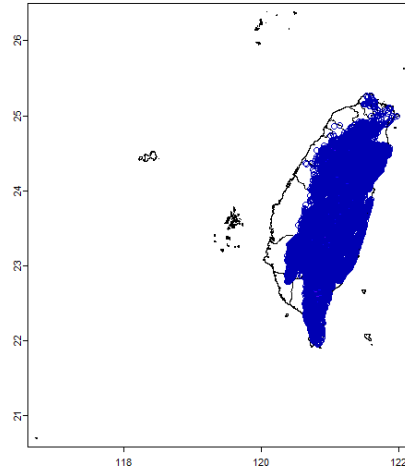
Taiwan landslide area prediction: Gradient boosting regression Class project for Geo-scripting
