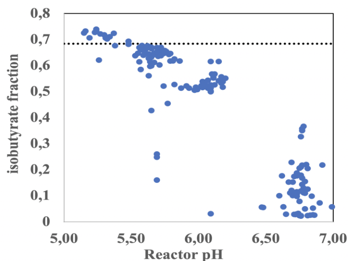
Fig. 1. Isobutyrate formation in an open-culture bio-reactor at different pH values.
