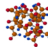
free metal ion fulvic acid
