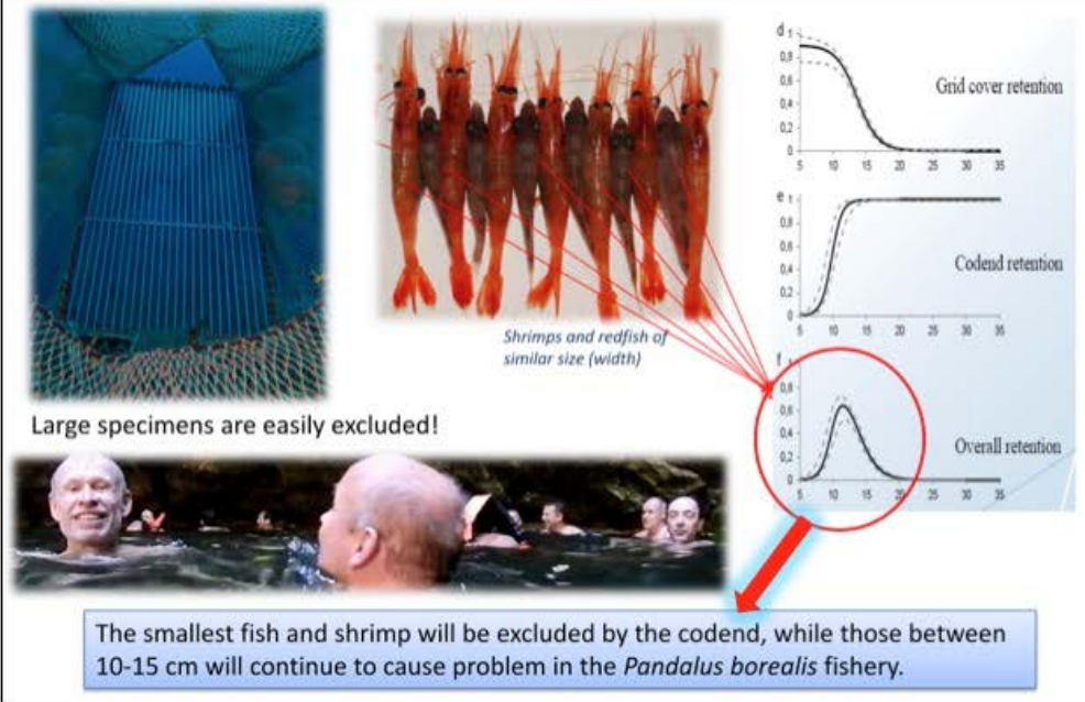
Figure 10.4.1. Summary of presentation, given by Roger B. Larsen (The Arctic University of Norway; Norway): Norwegian selectivity experiments (e.g. grid systems) and Contact probability as a driving factor for success.
